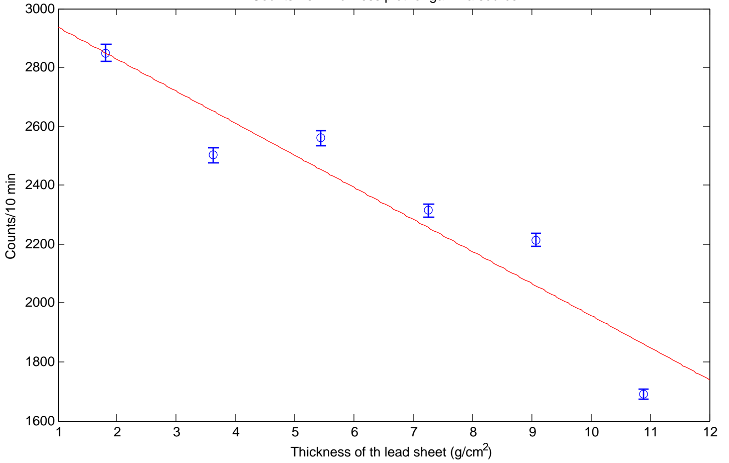
Counts Vs. Thickness plot for gamma source
