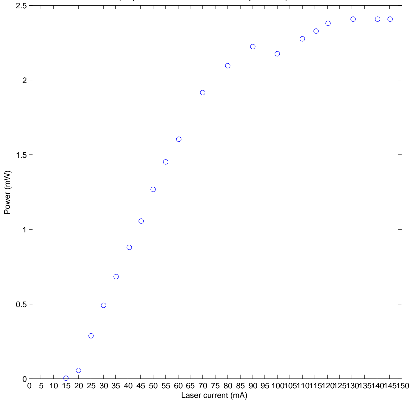
Output power of laser diode measured by external photodiode
