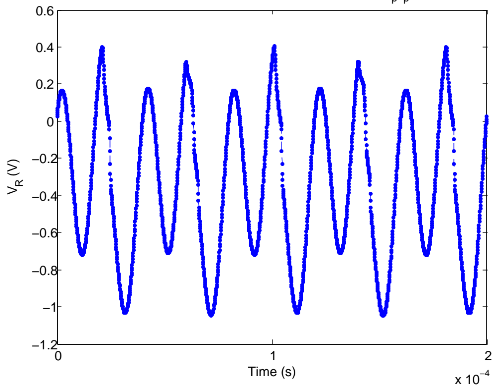
Onset of Period 4–Time series (at 16.3 V_{p-p} )
