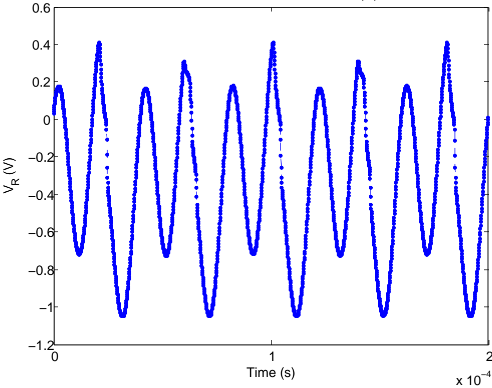
Period 4–Time series (at 16.5 V_{p-p} )
