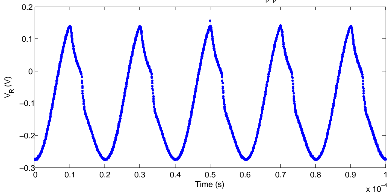
Period 1 – Time Series (at 4.9 V_{p-p} )
