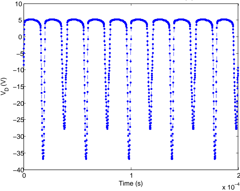
Onset of Period 2–Time series (at 4 V_{p-p} )
