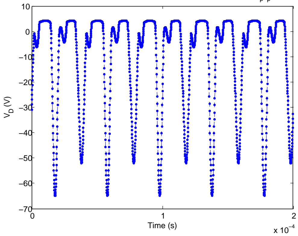
Period 2 with DC Offset of -1 V-Time series (at 4.3 V_{p-p} )
