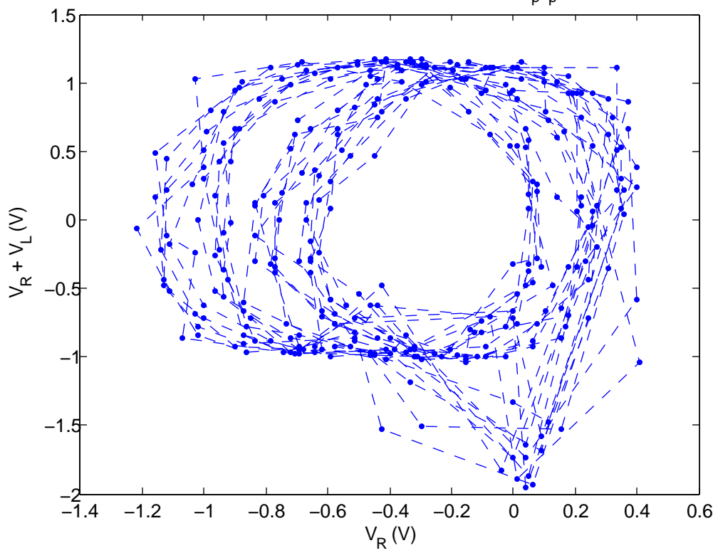
Period 4-Phase Portrait (at 16.7 V_{p-p} )
