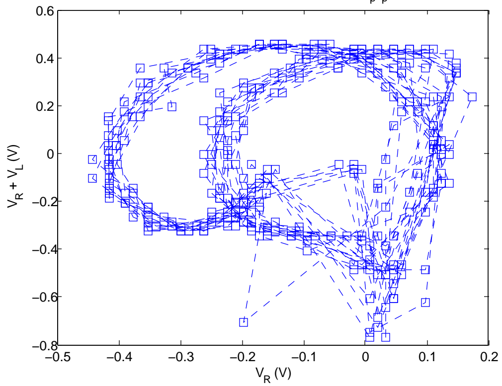
Period 2 – Phase Portait (at 6.3 V_{p-p} )
