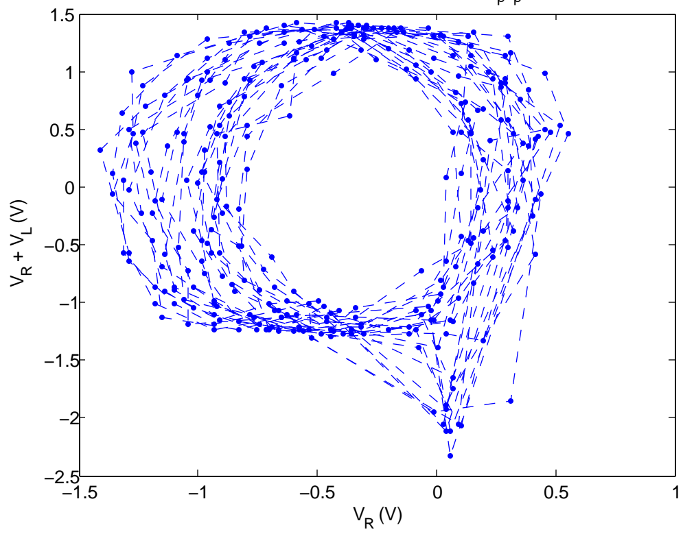
Chaos-Phase Portrait (at 20 V_{p-p} )
