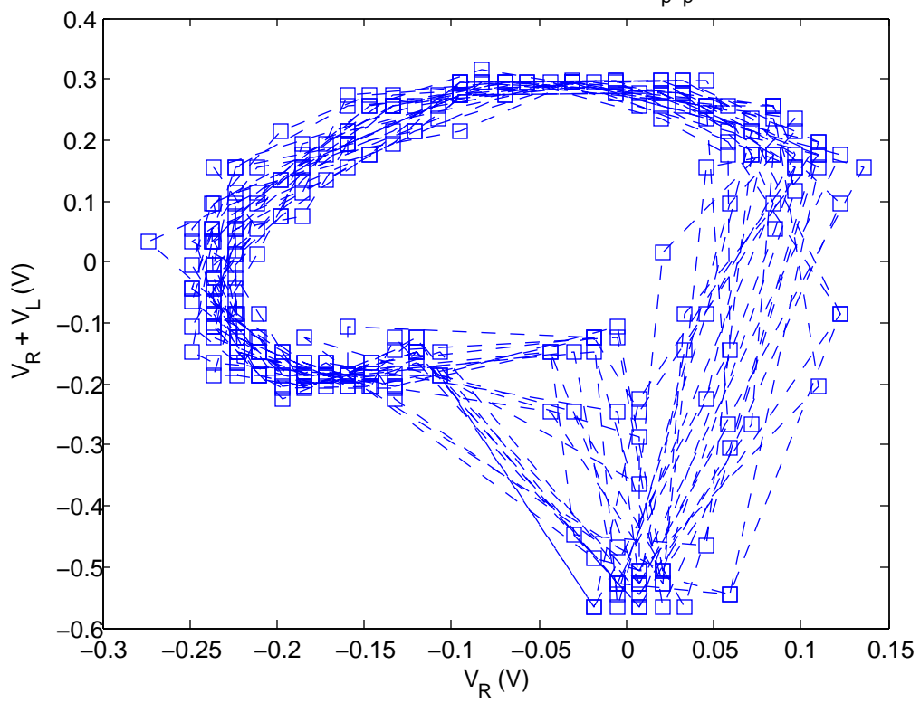
Period 1 – Phase Portait (at 4 V_{p-p} )
