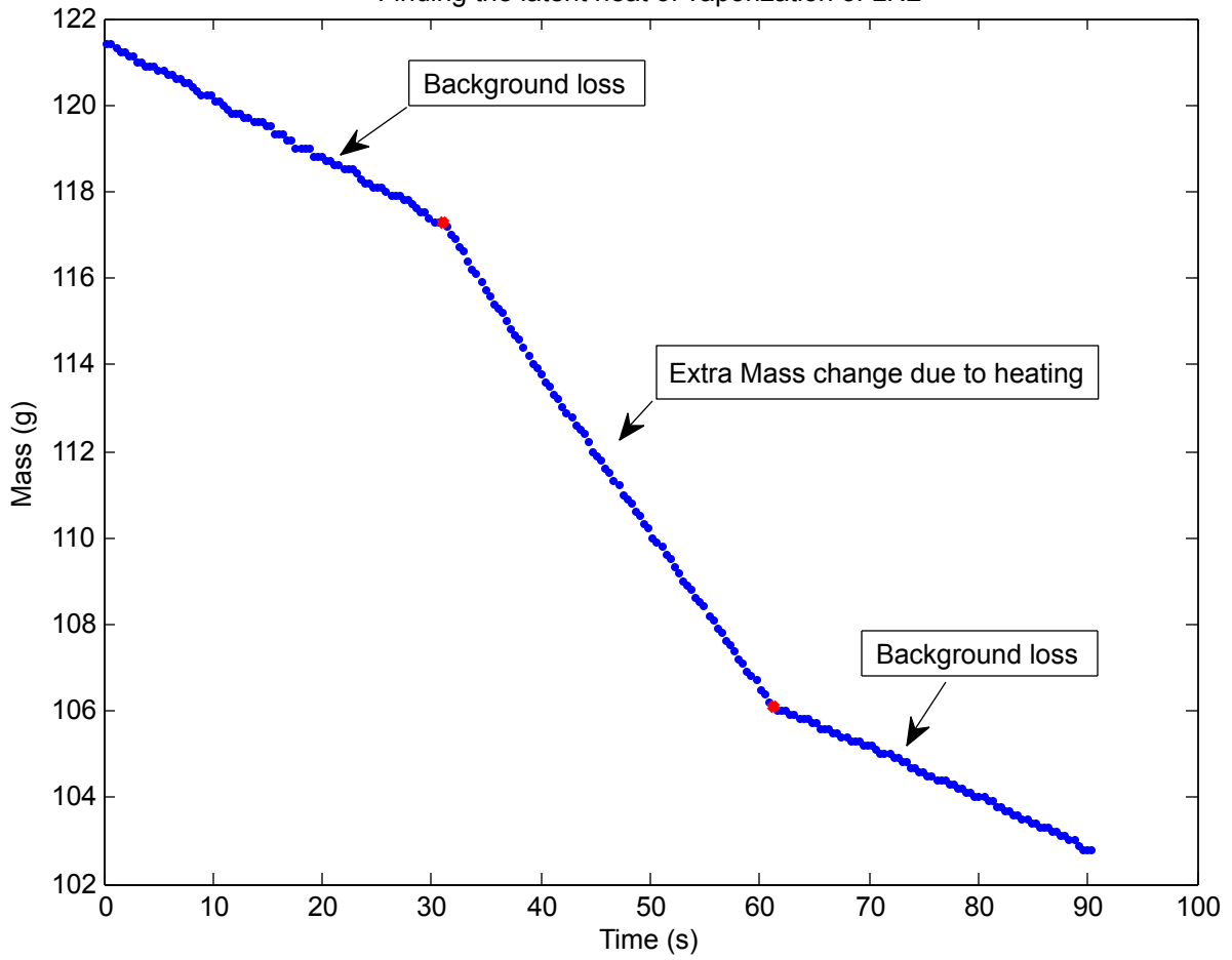
Finding the latent heat of vaporization of LN2
