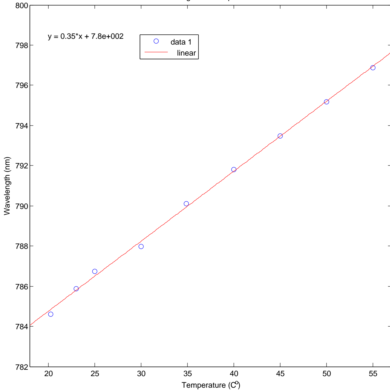
Variation of wavelength with temperature of laser diode
