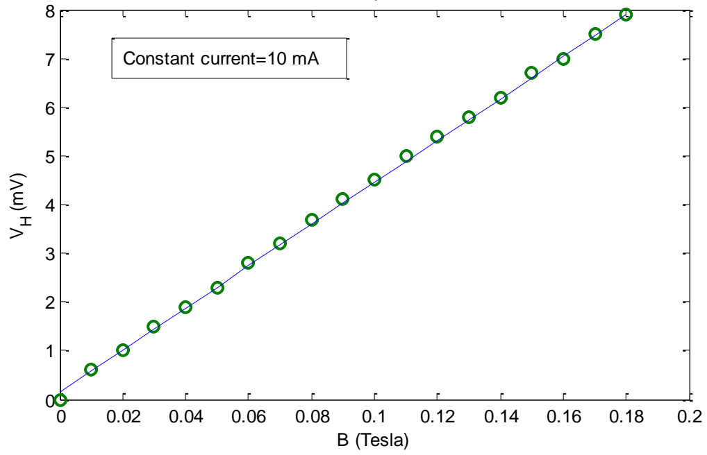
Graph of applied magnetic Field and Hall voltage at constant current through the crystal.
